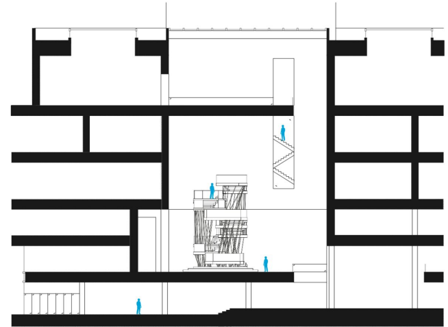
ELEVATION G INCLUDING SITE CONTEXT SCALE 1/8"=1'
